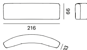
one-sided backrest M - only for Curve moduls
